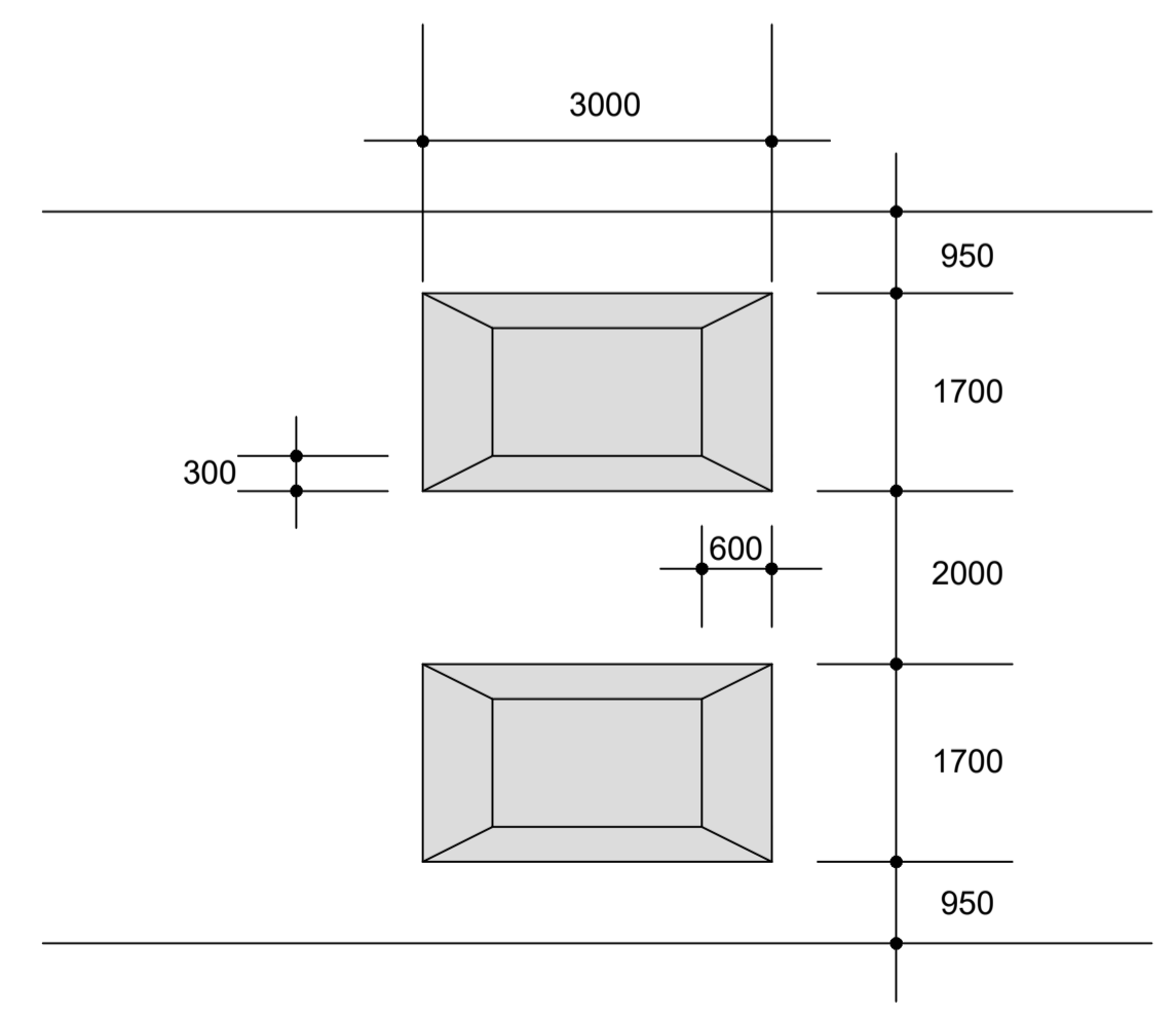
SPEED CUSHION DETAIL n.t.s
